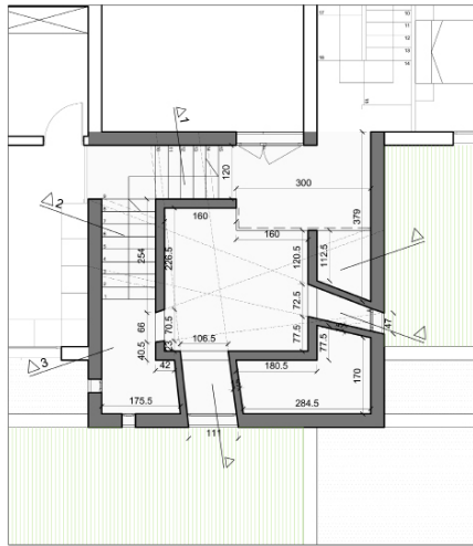
PLAN R+1
